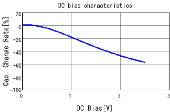
■ GRM188R60E476ME15 C-DC bias capchange, 25.0degC, ACO.
