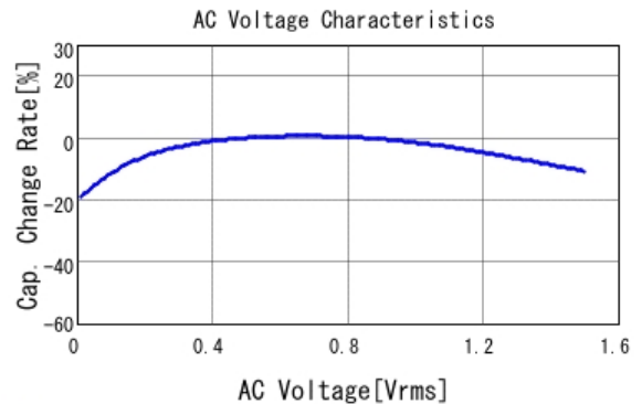
■ GRM188R60E476ME15 C-AC Voltage capchange, DCOV, 25.0d
