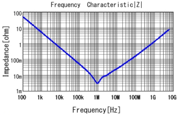
■ GRM188R60E476ME15 |Z| DCOV, 25degC
