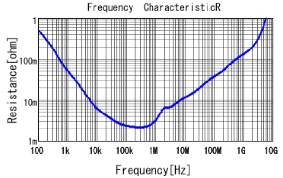
■ GRM188R60E476ME15 R DCOV, 25degC
