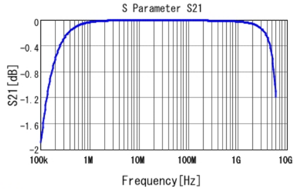
■ GRM188R11H223KA01 S21 DC0V, 20degC
