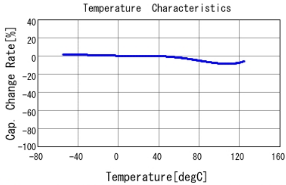
■ GRM188R11H223KA01 C-Temp. capchange, DC0.0V, AC1.0V rm
