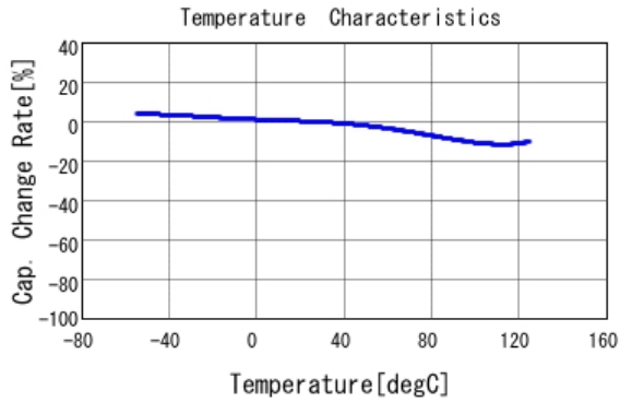
■ GRM188R11E473KA01 C-Temp. capchange, DC0.0V, AC1.0V rm
