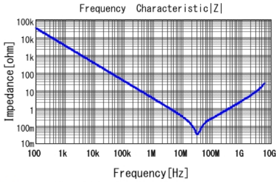
■ GRM188R11E473KA01 |Z| DCOV, 20degC
