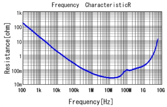
■ GRM188R11E473KA01 R DCOV, 20degC
