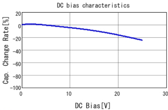
■ GRM188R11E473KA01 C-DC bias capchange, 20.0degC, AC1.
