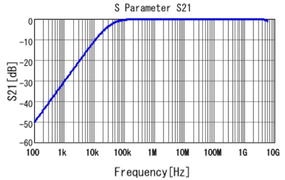
■ GRM188R11E473KA01 S21 DC0V, 20degC
