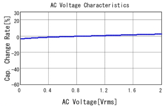
■ GRM188R11E473KA01 C-AC Voltage capchange, DCOV, 20.0d
