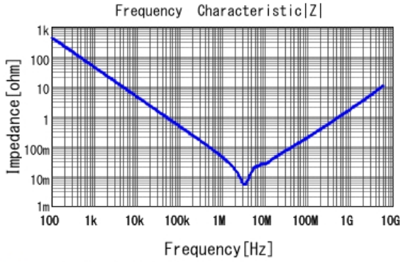
■ GRM188C81E475ME11 |Z| DCOV, 25degC
