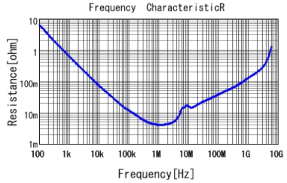
■ GRM188C81E475ME11 R DCOV, 25degC
