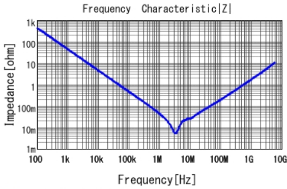
■ GRM188C81E475KE11 |Z| DCOV, 25degC
