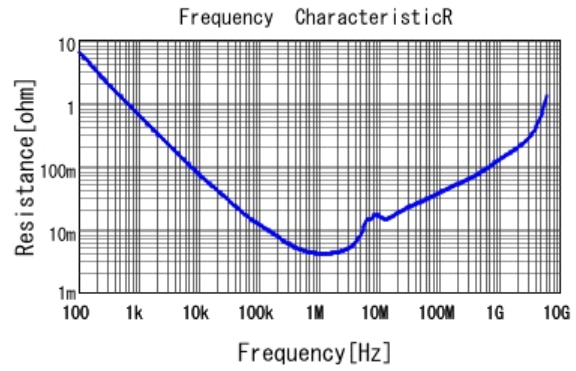
■ GRM188C81E475KE11 R DCOV, 25degC
