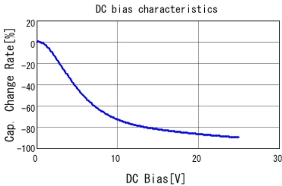
■ GRM188C81E475KE11 C-DC bias capchange, 25.0degC, AC1V
