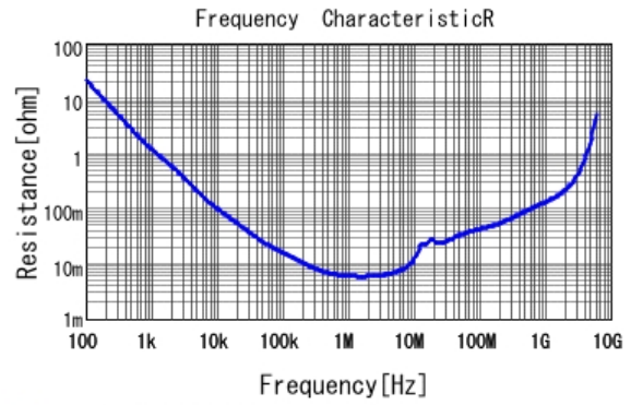
■ GRM188C81E105KAAD R DCOV, 25degC
