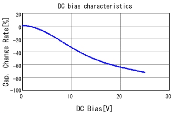
■ GRM188C81E105KAAD C-DC bias capchange, 25.0degC, AC1.
