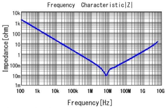
■ GRM188C81E105KAAD |Z| DCOV, 25degC
