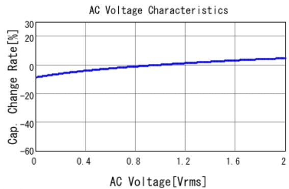
■ GRM188C81E105KAAD C-AC Voltage capchange, DCOV, 25.0d
