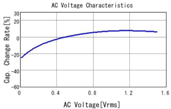
■ GRM188C80G106ME47 C-AC Voltage capchange, DCOV, 25.0d
