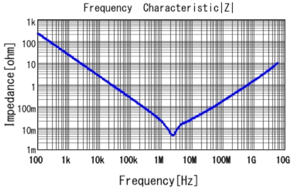
■ GRM188C80G106ME47 |Z| DCOV, 25degC
