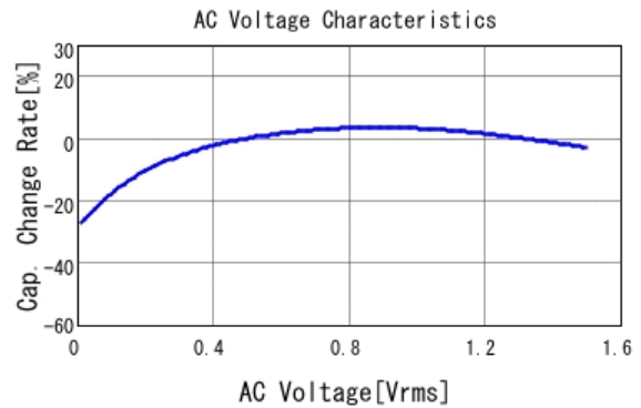
■ GRM188C60J226MEA0 C-AC Voltage capchange, DCOV, 25.0d
