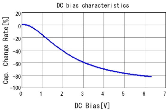
■ GRM188C60J226MEA0 C-DC bias capchange, 25.0degC, AC0.
