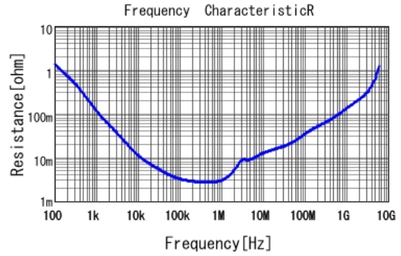
■ GRM188C60J226MEA0 R DCOV, 25degC
