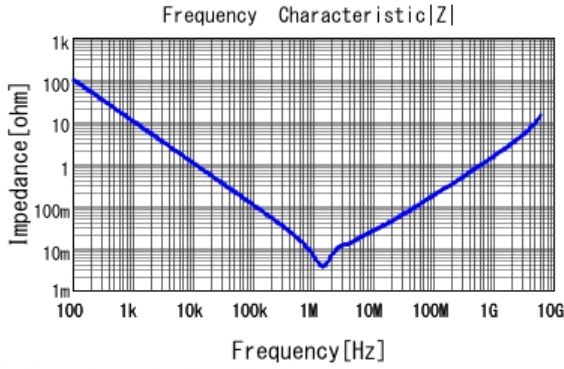
■ GRM188C60J226MEA0 |Z| DCOV, 25degC
