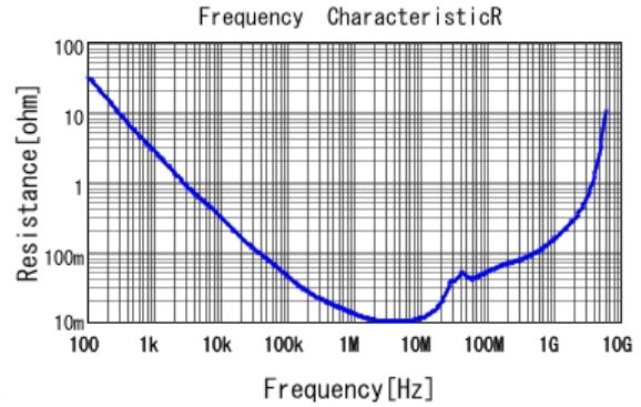
■ GRM188B31H224KAC4 R DCOV, 20degC
