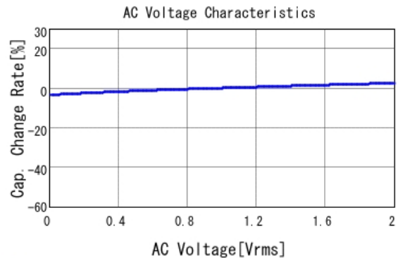
■ GRM188B31H224KAC4 C-AC Voltage capchange, DCOV, 20.0d
