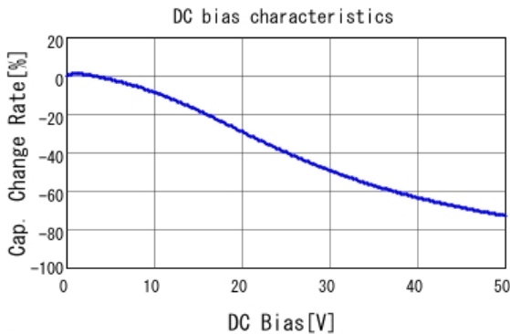
■ GRM188B31H224KAC4 C-DC bias capchange, 20.0degC, AC1.
