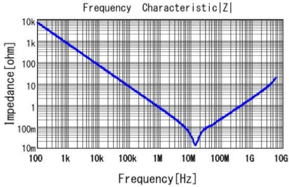
■ GRM188B31H224KAC4 |Z| DCOV, 20degC
