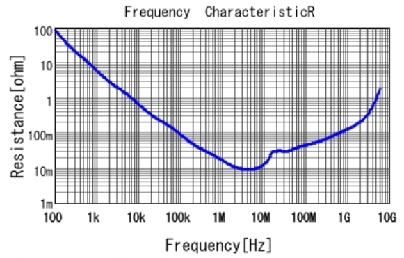
■ GRM188B31H105KAAL R DCOV, 20degC
