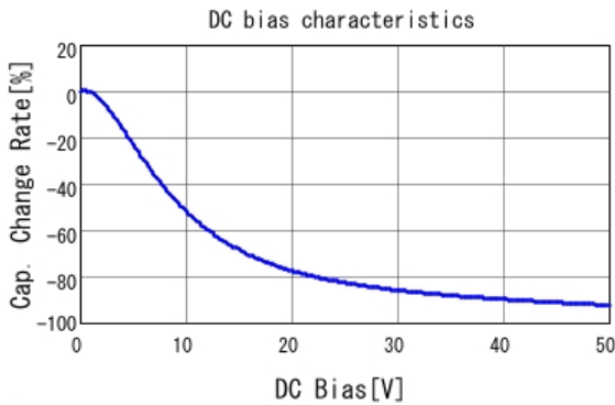
■ GRM188B31H105KAAL C-DC bias capchange, 20.0degC, AC1.
