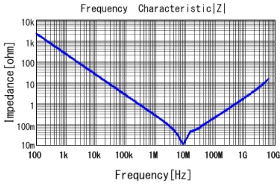
■ GRM188B31H105KAAL |Z| DCOV, 20degC
