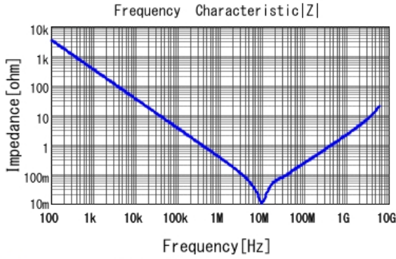
■ GRM188B31C474KA87 |Z| DCOV, 20degC
