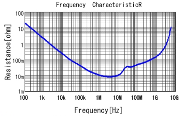
■ GRM188B31C474KA87 R DCOV, 20degC
