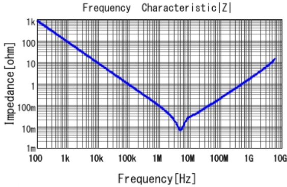
■ GRM188B31C225KE14 |Z| DCOV, 20degC
