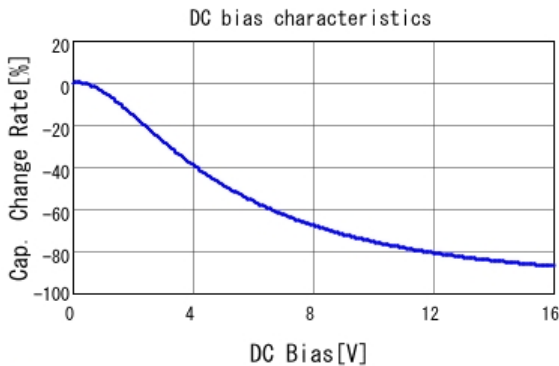
■ GRM188B31C225KE14 C-DC bias capchange, 20.0degC, AC0.
