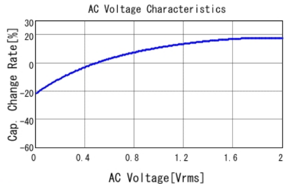
■ GRM188B31C225KE14 C-AC Voltage capchange, DCOV, 20.0d
