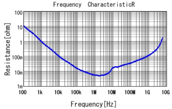
■ GRM188B31C225KE14 R DCOV, 20degC
