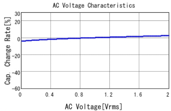
■ GRM188B11H223KA01 C-AC Voltage capchange, DCOV, 20.0d
