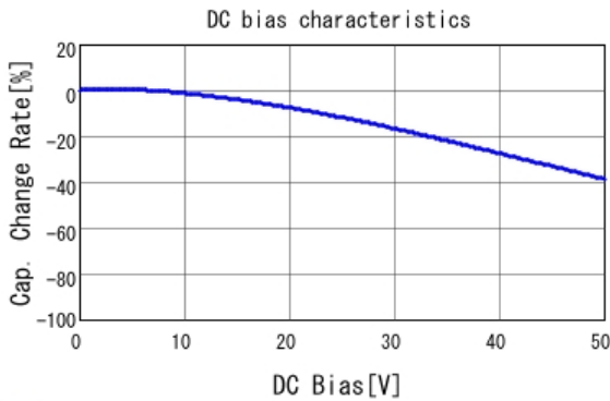
■ GRM188B11H223KA01 C-DC bias capchange, 20.0degC, AC1.
