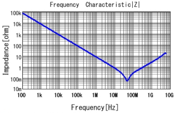
■ GRM188B11H223KA01 |Z| DCOV, 20degC
