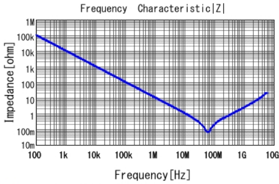
■ GRM188B11H153KA01 |Z| DCOV, 20degC
