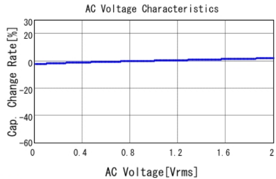
■ GRM188B11H153KA01 C-AC Voltage capchange, DCOV, 20.0d
