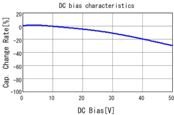
■ GRM188B11H153KA01 C-DC bias capchange, 20.0degC, AC1.
