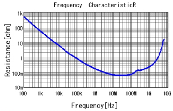
■ GRM188B11H153KA01 R DCOV, 20degC
