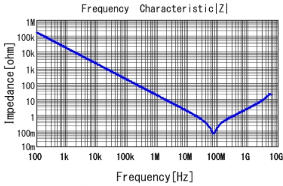
■ GRM188B11H103KA01 |Z| DCOV, 20degC
