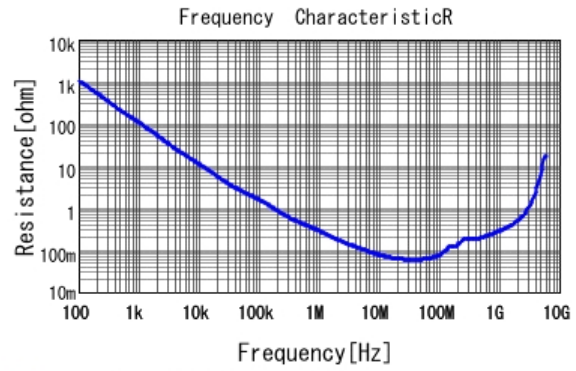
■ GRM188B11H103KA01 R DCOV, 20degC
