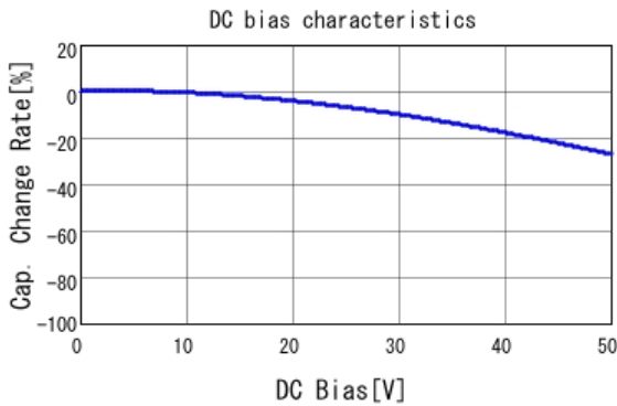
■ GRM188B11H103KA01 C-DC bias capchange, 20.0degC, AC1.
