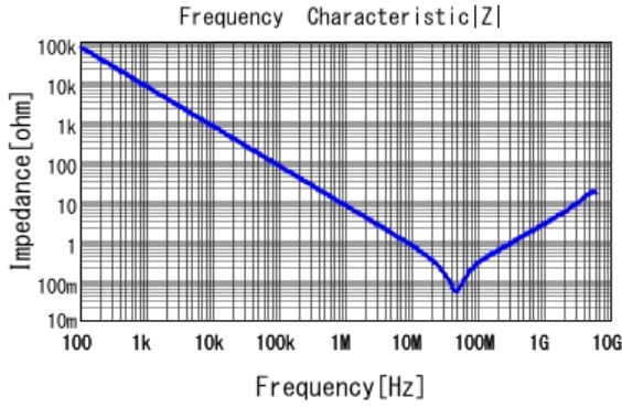
■ GRM188B11E223KA01 |Z| DCOV, 20degC
