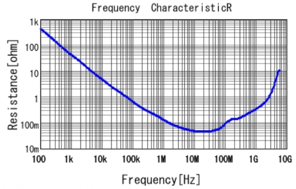
■ GRM188B11E223KA01 R DCOV, 20degC
