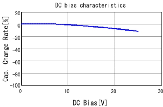
■ GRM188B11E223KA01 C-DC bias capchange, 20.0degC, AC1.
