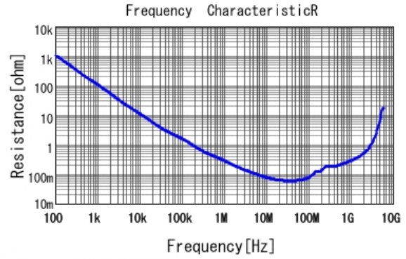
■ GRM188B11E103KA01 R DCOV, 20degC
