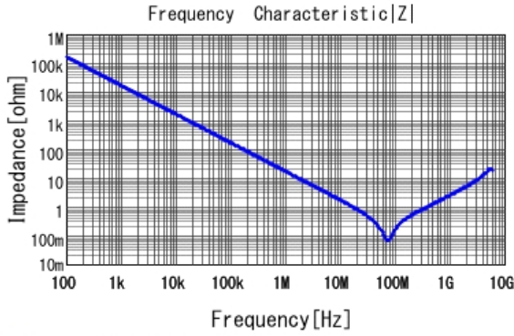
■ GRM188B11E103KA01 |Z| DCOV, 20degC
