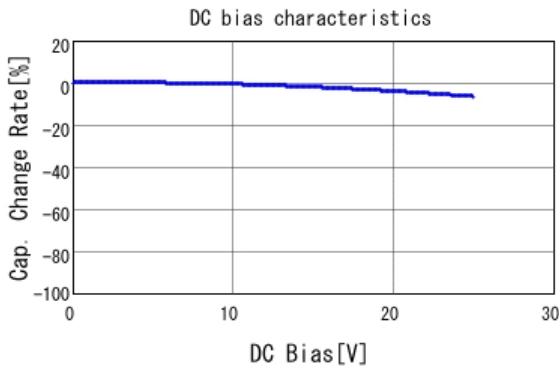
■ GRM188B11E103KA01 C-DC bias capchange, 20.0degC, AC1.
