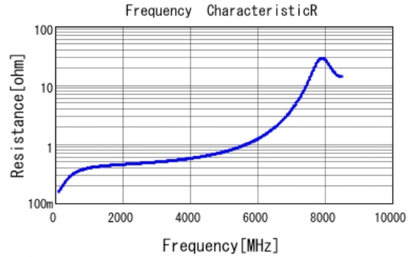
■ GRM1885C2A3R5BA01 R DCOV, 25degC
