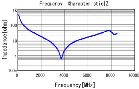
■ GRM1885C2A3R5BA01 |Z| DCOV, 25degC
