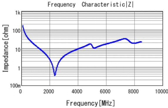
■ GRM1885C1H9R3DA01 |Z| DCOV, 25degC
