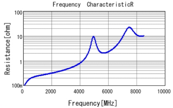
■ GRM1885C1H9R3DA01 R DCOV, 25degC
