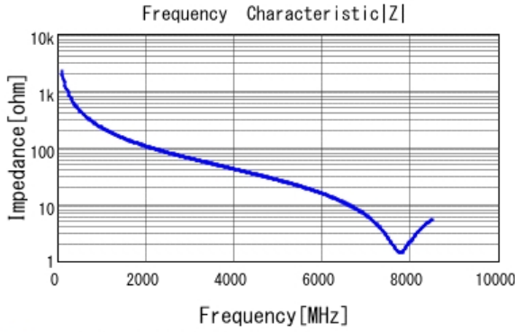
■ GRM1885C1HR70BA01 |Z| DCOV, 25degC
