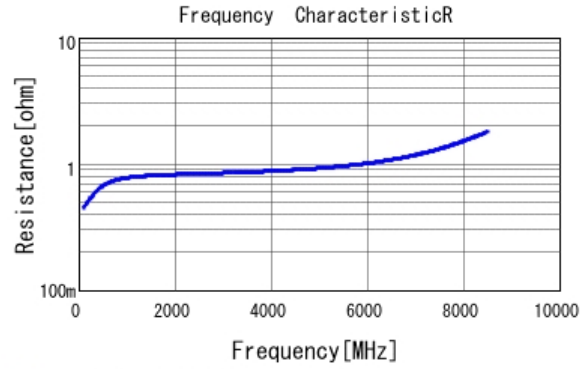
■ GRM1885C1HR70BA01 R DCOV, 25degC
