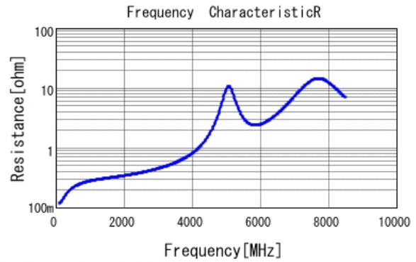
■ GRM1885C1H8R7CA01 R DCOV, 25degC
