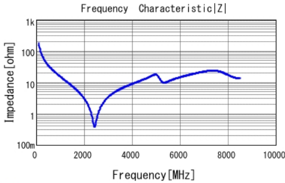
■ GRM1885C1H8R7CA01 |Z| DCOV, 25degC
