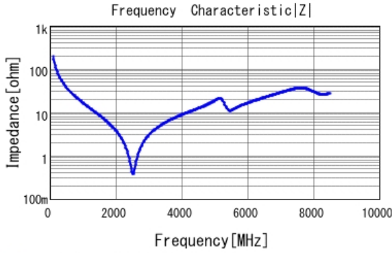
■ GRM1885C1H8R0BA01 |Z| DCOV, 25degC
