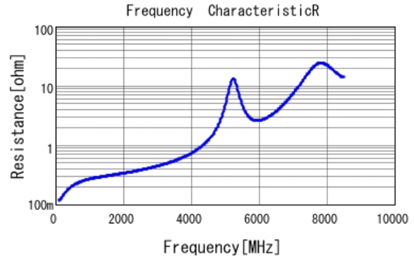
■ GRM1885C1H8R0BA01 R DCOV, 25degC
