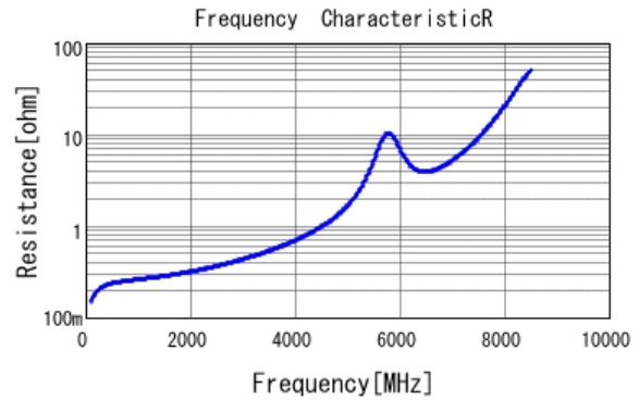
■ GRM1885C1H7R1BA01 R DCOV, 25degC
