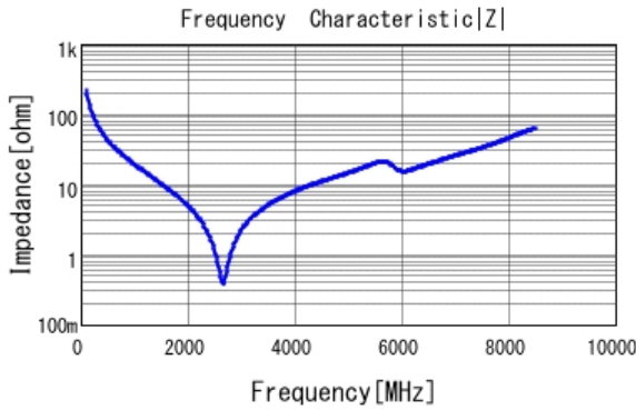
■ GRM1885C1H7R1BA01 |Z| DCOV, 25degC
