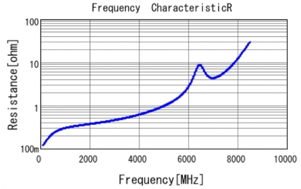
■ GRM1885C1H6R2BA01 R DCOV, 25degC
