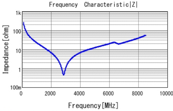
■ GRM1885C1H6R2BA01 |Z| DCOV, 25degC
