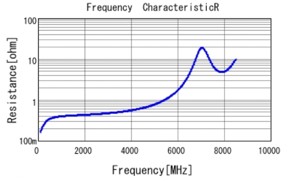
■ GRM1885C1H4R4CA01 R DCOV, 25degC
