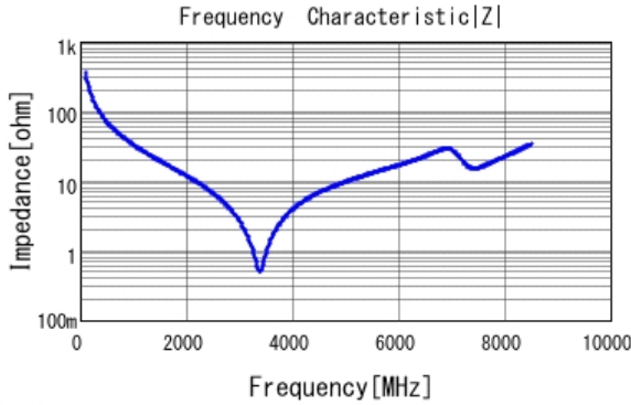
■ GRM1885C1H4R4CA01 |Z| DCOV, 25degC
