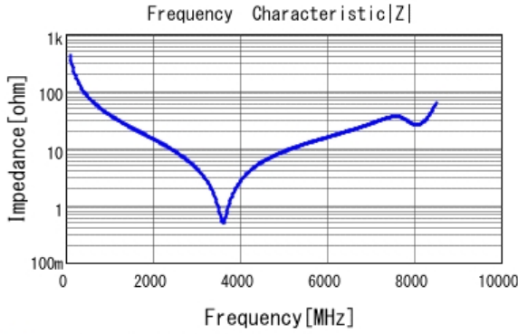
■ GRM1883C2A3R8BA01 |Z| DCOV, 20degC
