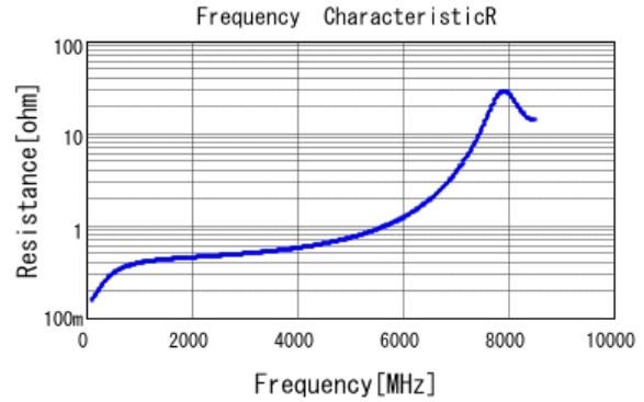
■ GRM1883C2A3R6BA01 R DCOV, 20degC
