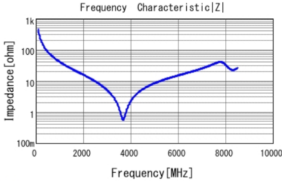
■ GRM1883C2A3R6BA01 |Z| DCOV, 20degC
