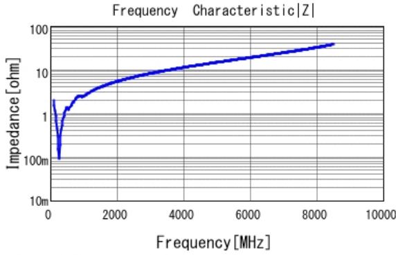
■ GRM1882C1H681JA01 |Z| DCOV, 20degC
