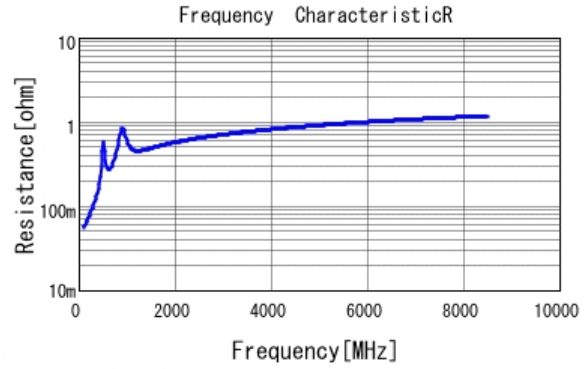
■ GRM1882C1H681JA01 R DCOV, 20degC
