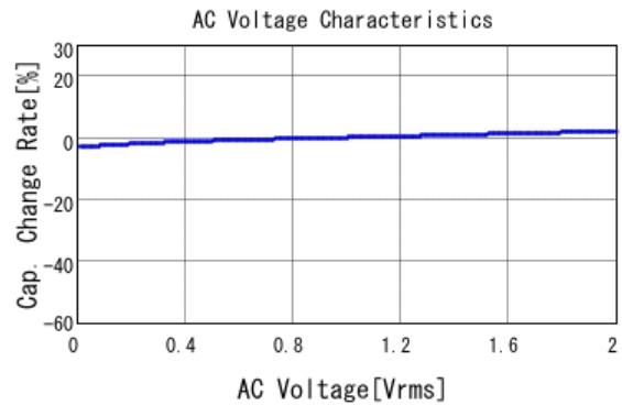
■ GRM155R71H102MA01 C-AC Voltage capchange, DCOV, 25.0d
