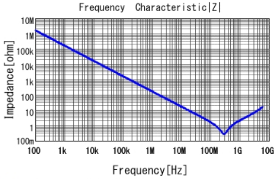
■ GRM155R71H102MA01 |Z| DCOV, 25degC
