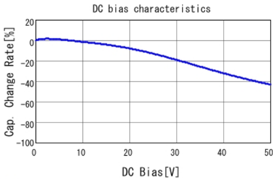
■ GRM155R71H102MA01 C-DC bias capchange, 25.0degC, AC1.
