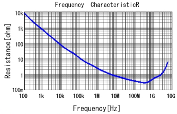
■ GRM155R71H102MA01 R DCOV, 25degC
