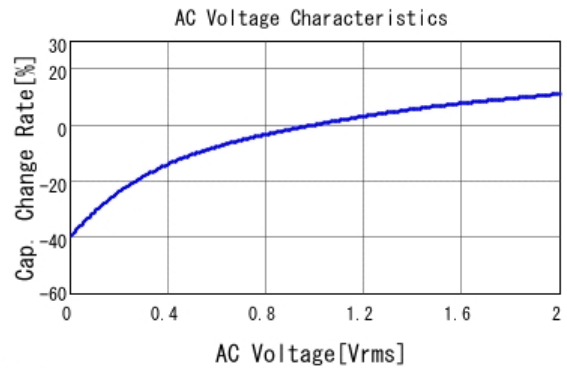
■ GRM155R71A224ME01 C-AC Voltage capchange, DCOV, 25.0d
