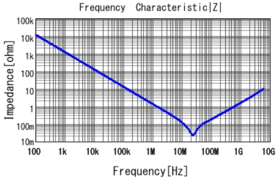
■ GRM155R71A224ME01 |Z| DCOV, 25degC
