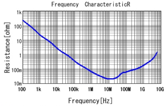
■ GRM155R71A224ME01 R DCOV, 25degC
