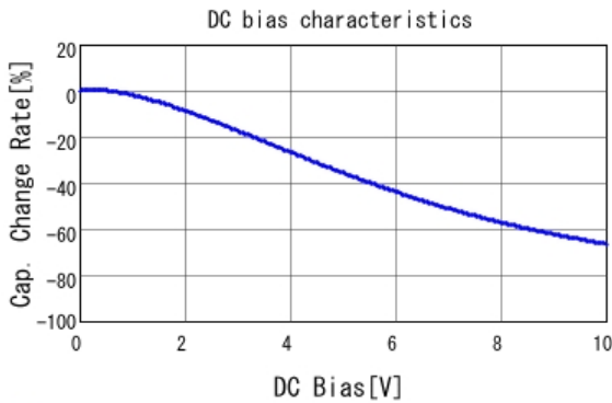
■ GRM155R61A684KE15 C-DC bias capchange, 25.0degC, AC0.
