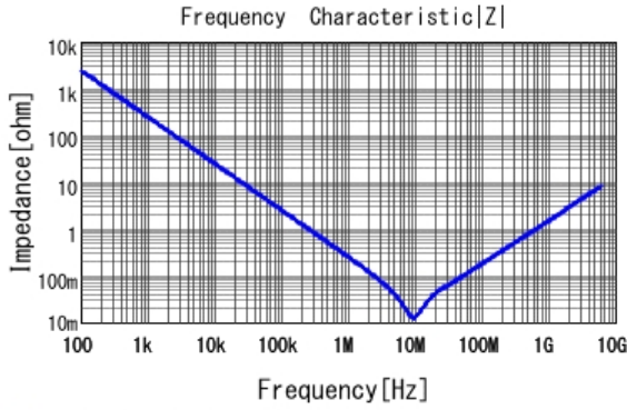
■ GRM155R61A684KE15 |Z| DCOV, 25degC
