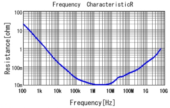
■ GRM155R61A684KE15 R DCOV, 25degC
