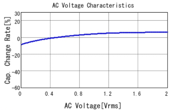
■ GRM155R61A684KE15 C-AC Voltage capchange, DCOV, 25.0d
