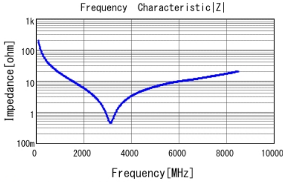
■ GRM1555C2A8R0DA01 |Z| DCOV, 25degC
