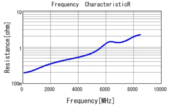
■ GRM1555C2A8R0DA01 R DCOV, 25degC
