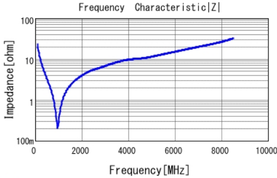
■ GRM1555C2A680JA01 |Z| DCOV, 25degC
