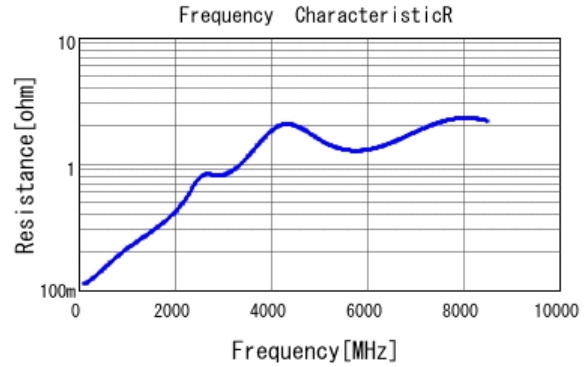
■ GRM1555C2A680JA01 R DCOV, 25degC
