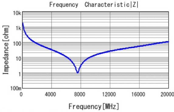
■ GRM1555C1HR90BA01 |Z| DC0V, 25degC
