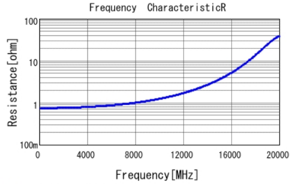
■ GRM1555C1HR90BA01 R DC0V, 25degC
