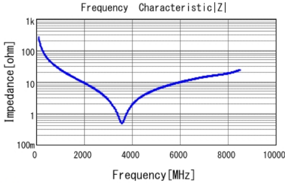
■ GRM1555C1H6R0BA01 |Z| DCOV, 25degC
