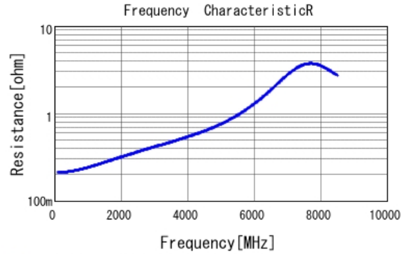
■ GRM1555C1H6R0BA01 R DCOV, 25degC
