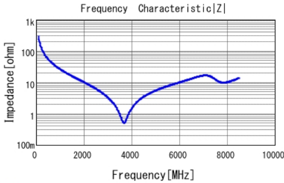
■ GRM1555C1H5R6WA01 |Z| DCOV, 25degC
