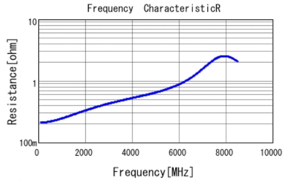
■ GRM1555C1H5R4WA01 R DCOV, 25degC
