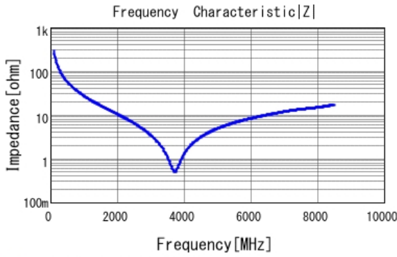
■ GRM1555C1H5R4WA01 |Z| DCOV, 25degC
