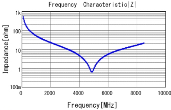
■ GRM1555C1H3R0BA01 |Z| DCOV, 25degC
