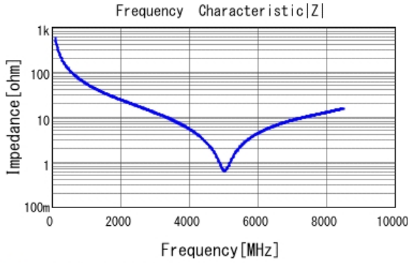
■ GRM1555C1H2R8BA01 |Z| DCOV, 25degC
