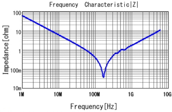
■ GRM1555C1H272JE01 |Z| DCOV, 25degC
