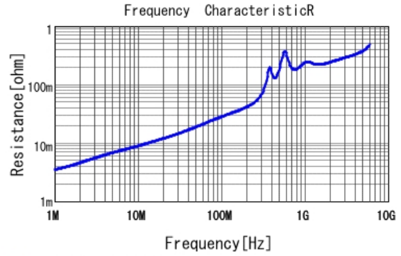
■ GRM1555C1H272JE01 R DCOV, 25degC
