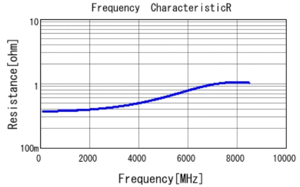
■ GRM1555C1E2R0CA01 R DCOV, 25degC
