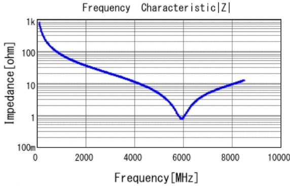
■ GRM1555C1E2R0CA01 |Z| DCOV, 25degC
