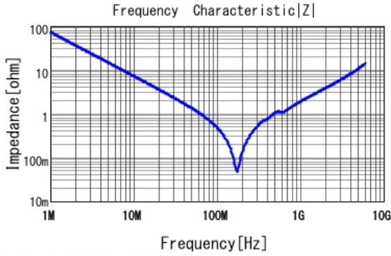
■ GRM1555C1E222JA01 |Z| DCOV, 25degC
