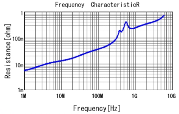
■ GRM1555C1E222JA01 R DCOV, 25degC
