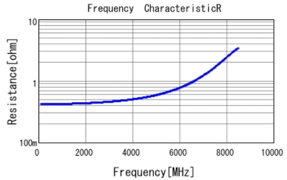
■ GRM1554C2A1R8WA01 R DCOV, 20degC
