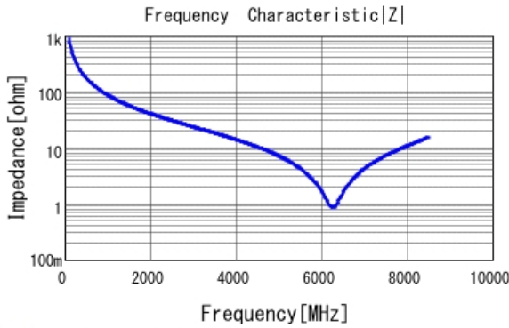
■ GRM1554C2A1R8WA01 |Z| DCOV, 20degC
