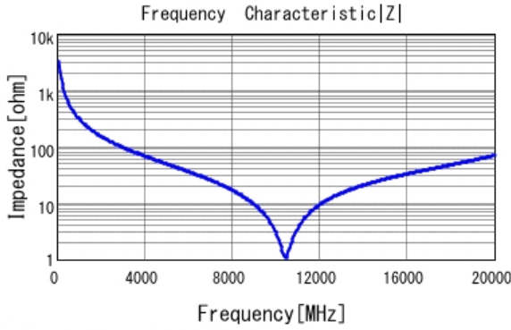
■ GRM1554C1HR50BA01 |Z| DCOV, 20degC
