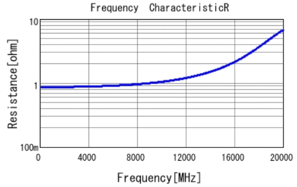
■ GRM1554C1HR50BA01 R DCOV, 20degC
