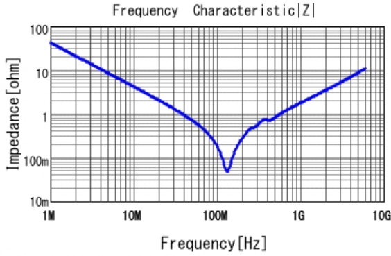
■ GRM1551X1A392JA01 |Z| DCOV, 20degC
