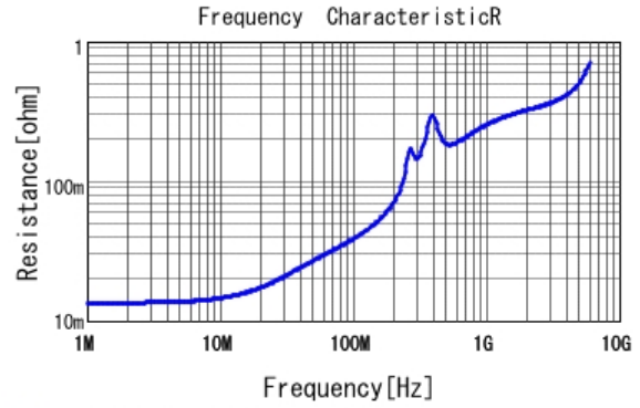
■ GRM1551X1A392JA01 R DCOV, 20degC
