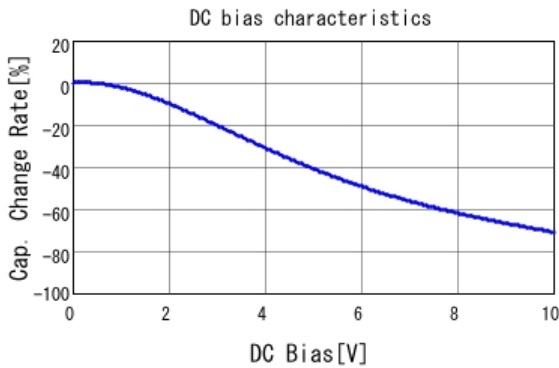
■ GRM152R61A224KE19 C-DC bias capchange, 25.0degC, AC1V
