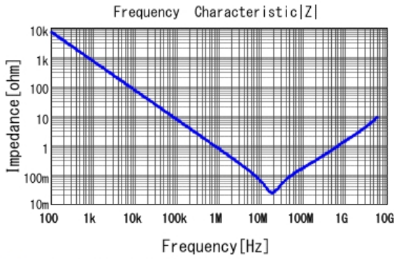
■ GRM152R61A224KE19 |Z| DCOV, 25degC
