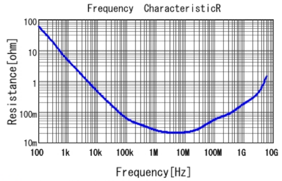
■ GRM152R61A224KE19 R DCOV, 25degC
