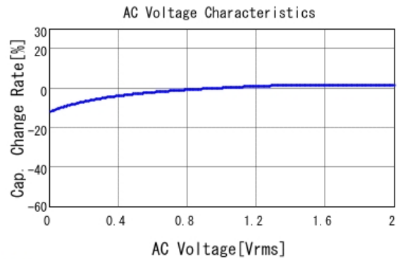
■ GRM152R61A224KE19 C-AC Voltage capchange, DCOV, 25.0d
