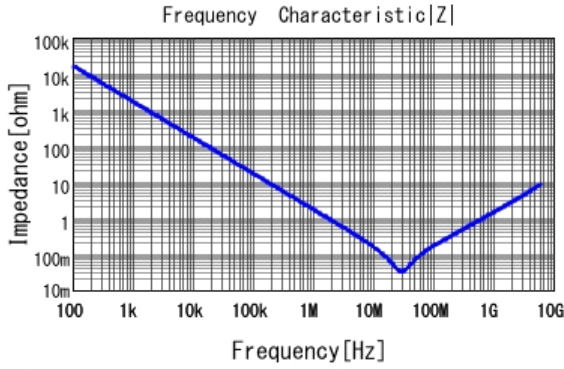
■ GRM152R61A104KE19 |Z| DCOV, 25degC
