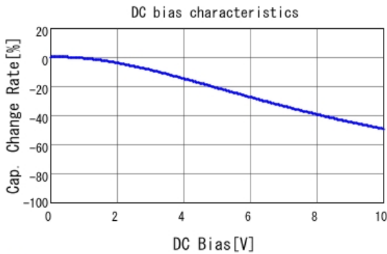
■ GRM152R61A104KE19 C-DC bias capchange, 25.0degC, AC1V
