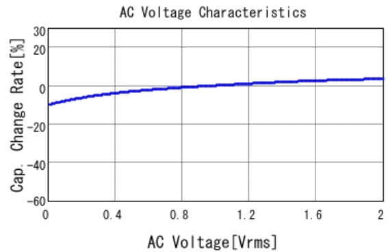
■ GRM152R61A104KE19 C-AC Voltage capchange, DCOV, 25.0d
