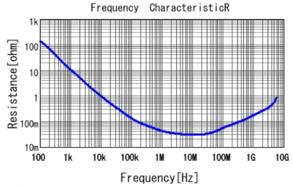
■ GRM152R61A104KE19 R DCOV, 25degC
