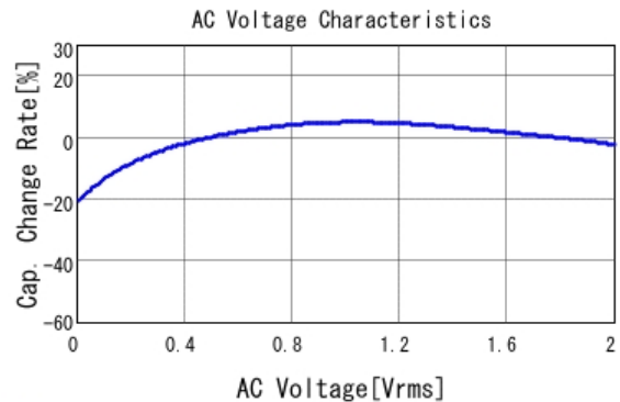
■ GRM152R60J474ME15 C-AC Voltage capchange, DCOV, 25.0d
