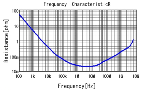
■ GRM152R60J474ME15 R DCOV, 25degC
