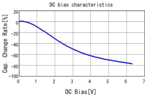
■ GRM152R60J474ME15 C-DC bias capchange, 25.0degC, ACO.
