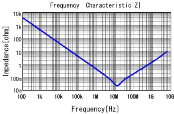
■ GRM152R60J474ME15 |Z| DCOV, 25degC
