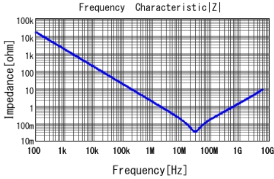
■ GRM152R60J104ME19 |Z| DCOV, 25degC
