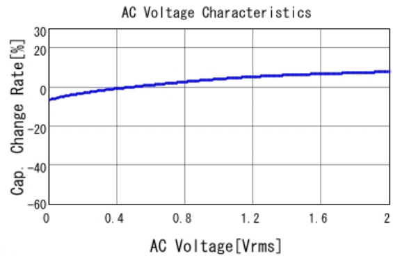
■ GRM152R60J104ME19 C-AC Voltage capchange, DCOV, 25.0d
