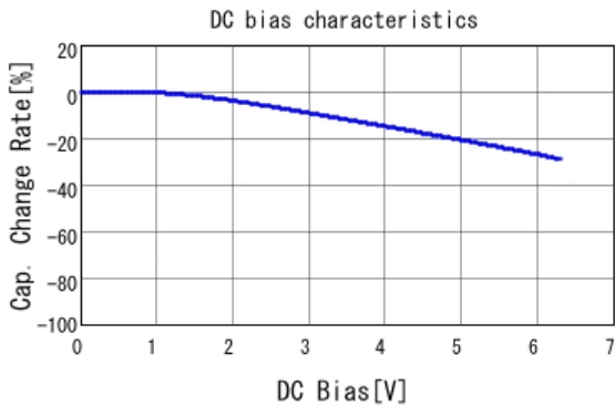
■ GRM152R60J104ME19 C-DC bias capchange, 25.0degC, ACO.
