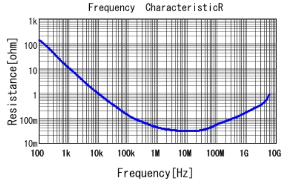
■ GRM152R60J104ME19 R DCOV, 25degC
