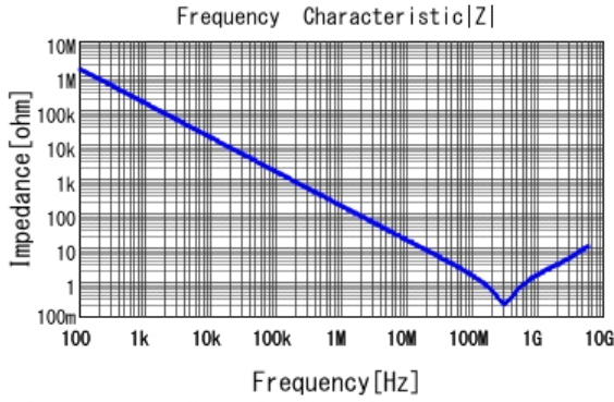
■ GRM033R71H102MA12 |Z| DCOV, 25degC
