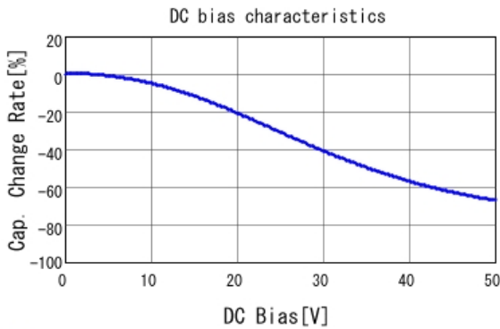
■ GRM033R71H102MA12 C-DC bias capchange, 25.0degC, AC1.
