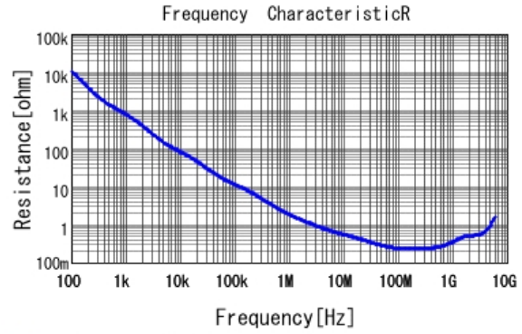
■ GRM033R71H102MA12 R DCOV, 25degC
